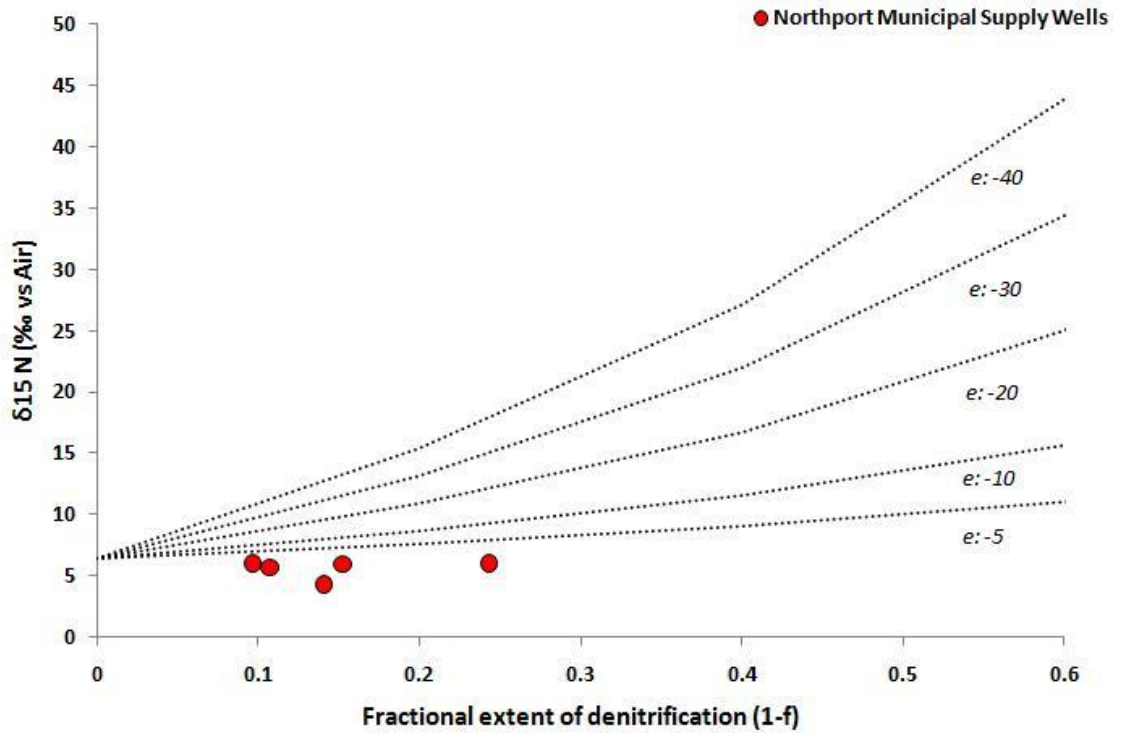
Figure 11 Nitrate \delta^{15}\text{N}\text{‰} vs fractional extent of denitrification (1-f) as determined from excess \text{N}_2 and residual nitrate in Northport supply well samples. Enrichment factors ( \epsilon ) ranging from 0 to -0.2 for five municipal supply wells. \delta^{15}\text{N}\text{‰} values from (BLEIFUSS et al., 2000). Dashed lines are typical denitrification enrichment factors, -5 to -40 (HUBNER, 1986) with initial \delta^{15}\text{N}\text{‰} of 6.4‰. The isotope data for Northport groundwater does not plot along enrichment trends due to lack of vadose zone denitrification.
